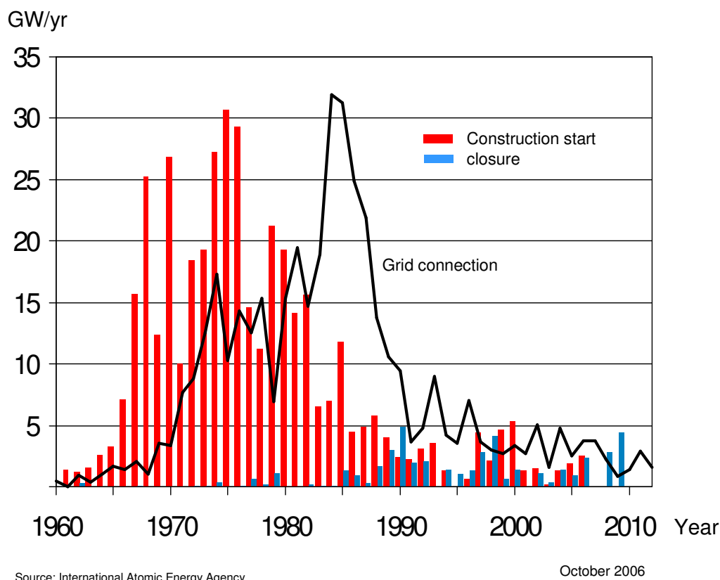
Figure 8: Construction start and decommissioning of nuclear power plants at world level
